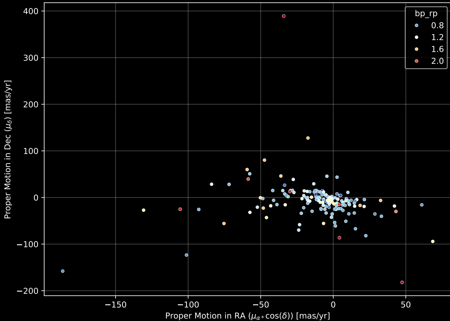
APOGEE DR17 Field: [041+50_MGA] Proper Motion Diagram (n= 157)
