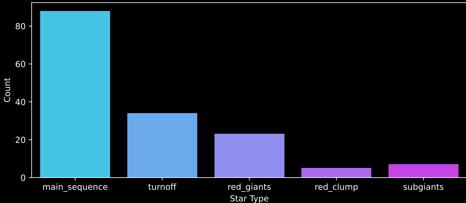
APOGEE DR17 Field: [041+50_MGA] Count plot of Star Type
