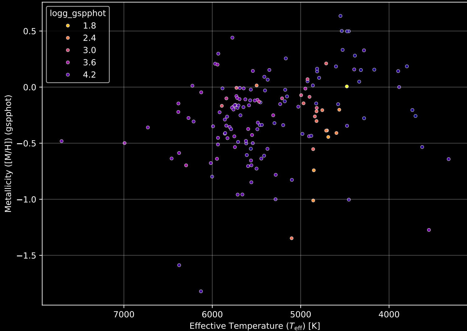
APOGEE DR17 Field: [041+50_MGA] Stellar Population Parameters (n= 157)
