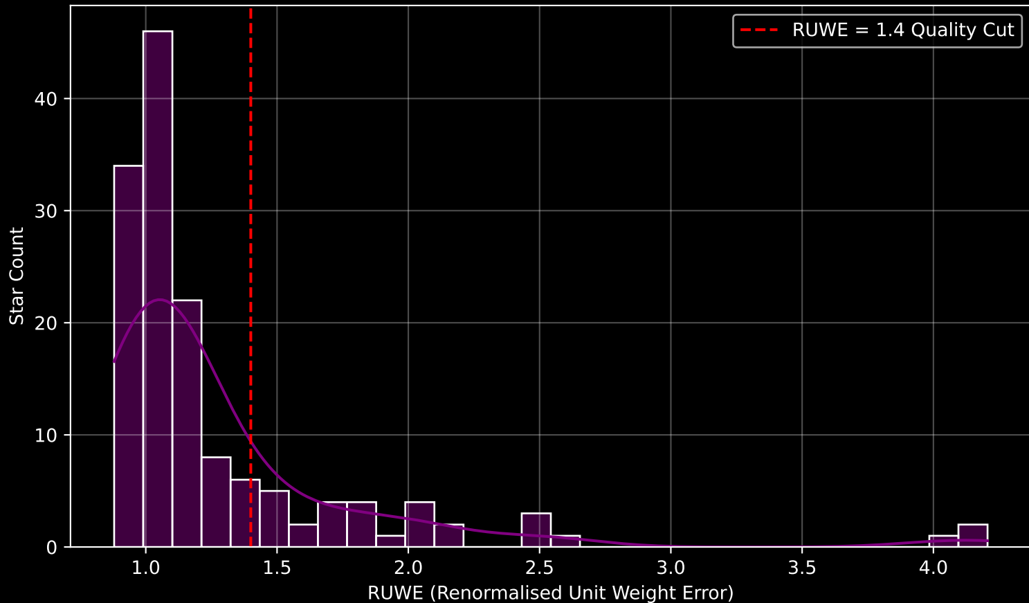
GAPOGEE DR17 Field [041+50_MGA] RUWE Distribution (n= 145)
