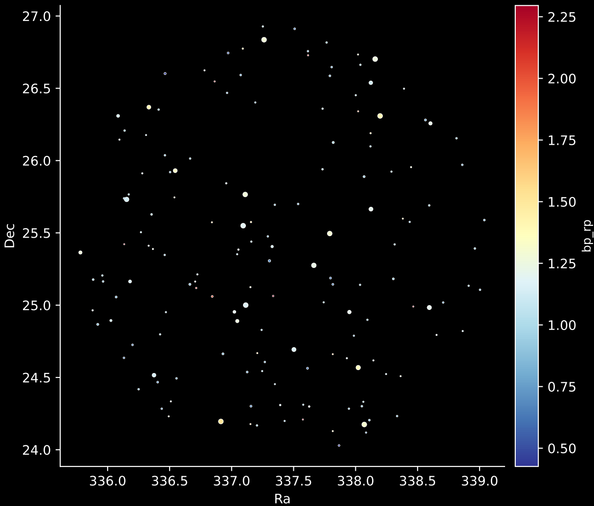
APOGEE DR17 Field: [041+50_MGA] Stars: 157
