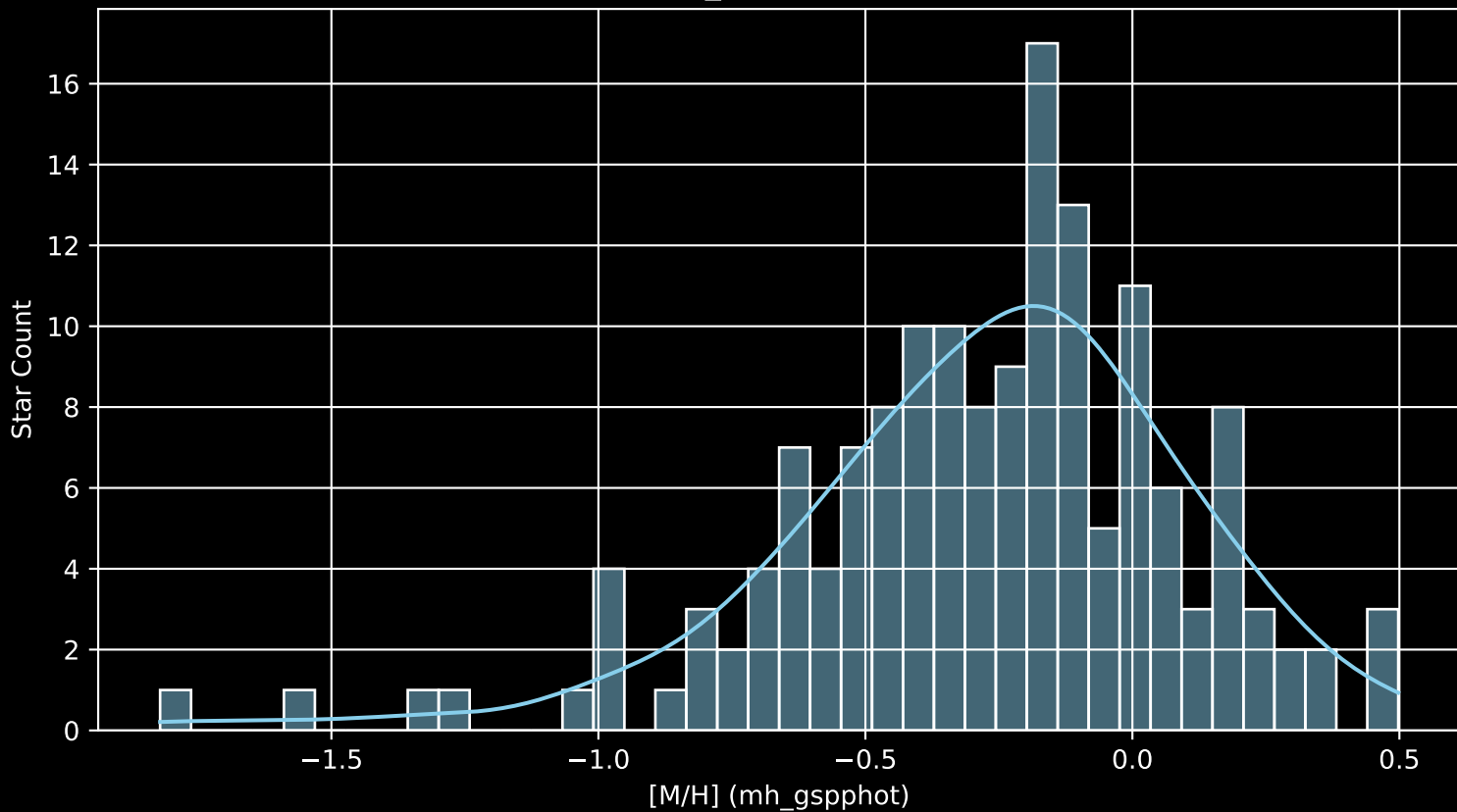
APOGEE DR17 Field: [041+50_MGA [M/H] (mh_gspphot) (n= 155)
