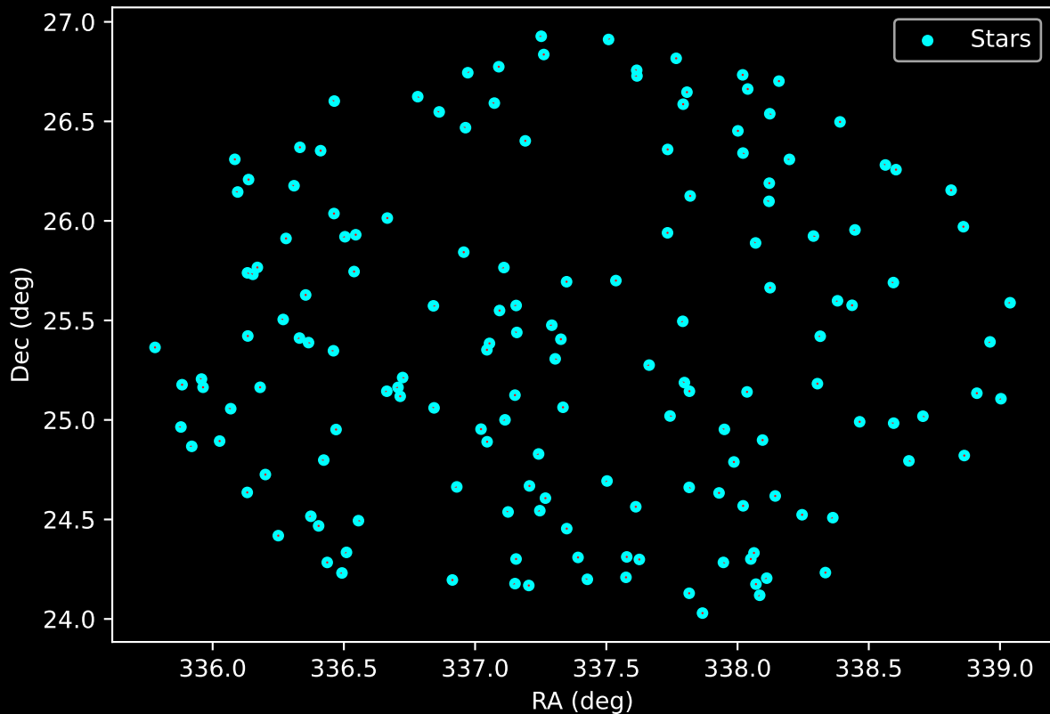
APOGEE DR17 Field: [041+50_MGA] Proper Motion Vectors for Gaia Star Field (n= 157)
