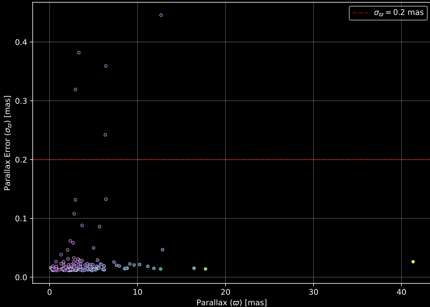
APOGEE DR17 Field: [041+50_MGA] Parallax Quality (n= 157)
